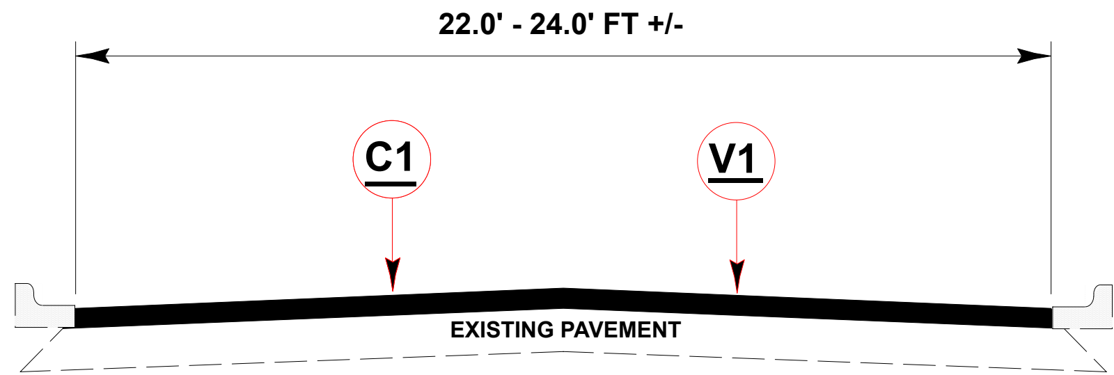
TYPICAL SECTION # 1 MAP(S) # 1, 7, & 8
